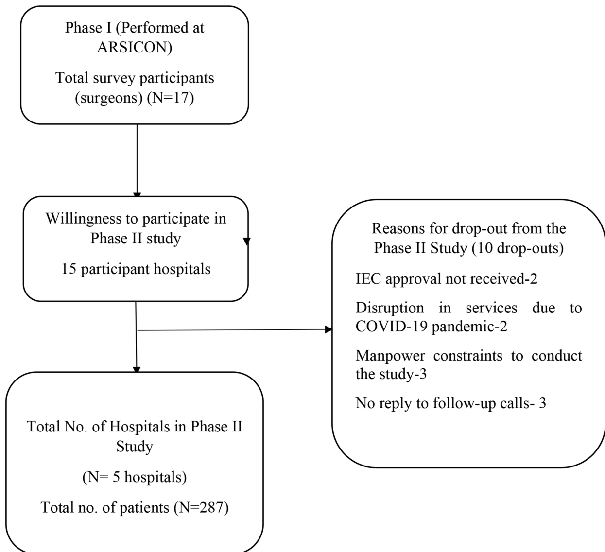
Fig. 1 Recruitment algorithm
